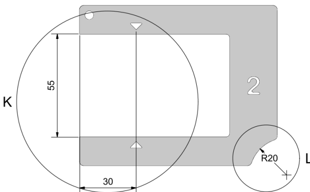
Figure 4 - Gauge 2
